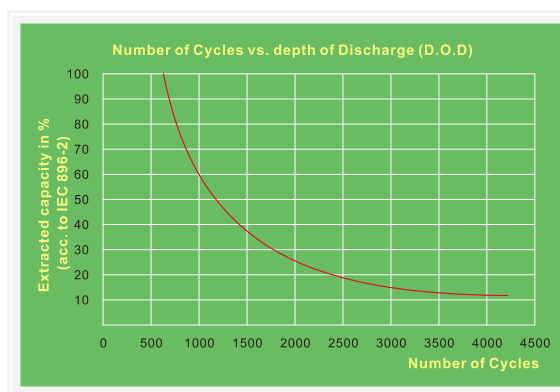
Cycle Life VS. DOD
